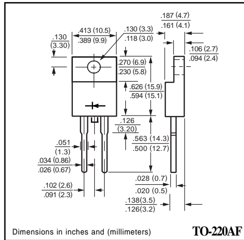
TO-220AF
