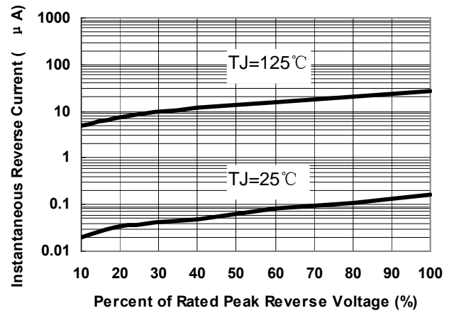
Fig.2-Typical Reverse Characteristics
