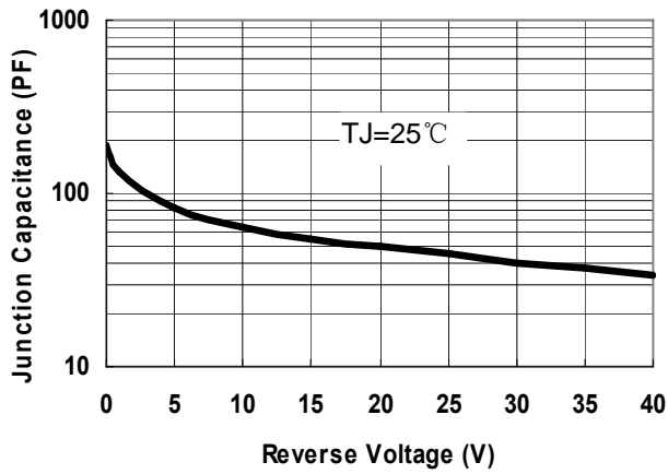
Fig.1-Typical Junction Capacitance
