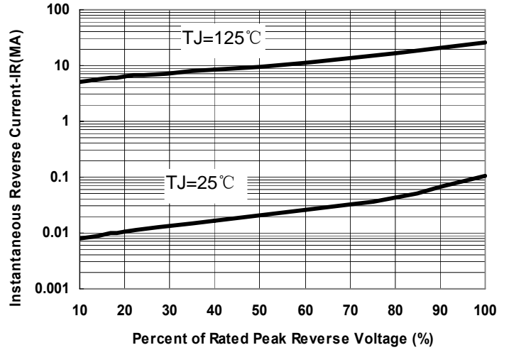
Fig.2-Typical Reverse Characteristics
