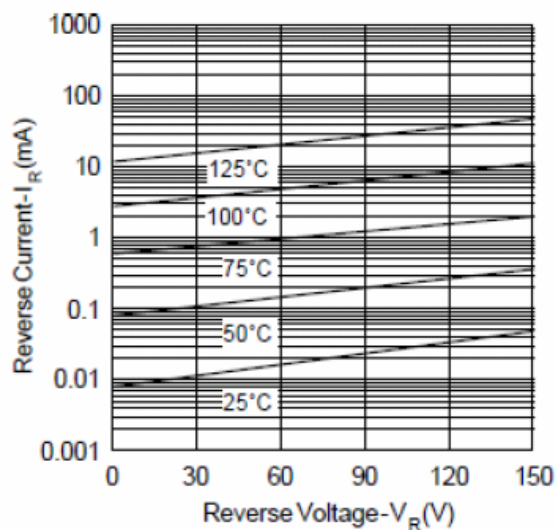
Fig.2-Typical Reverse Characteristics
