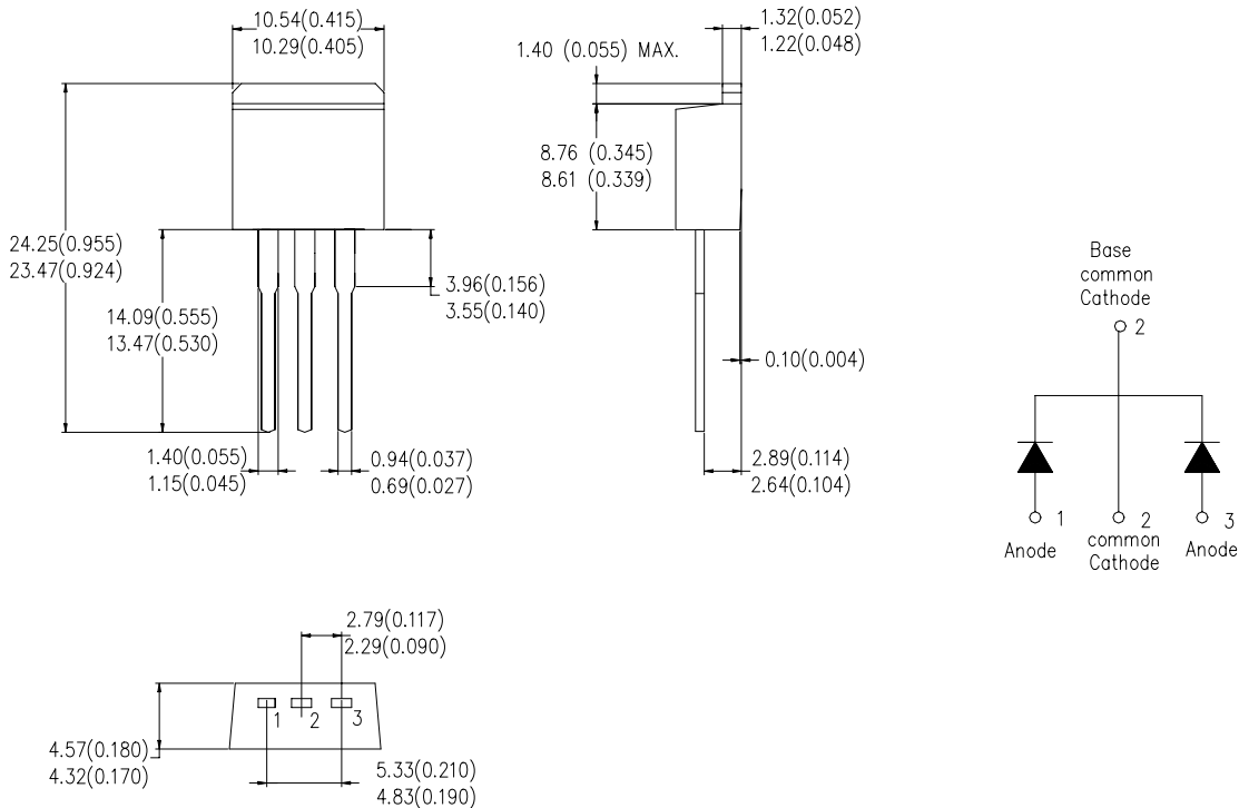
TO-262
