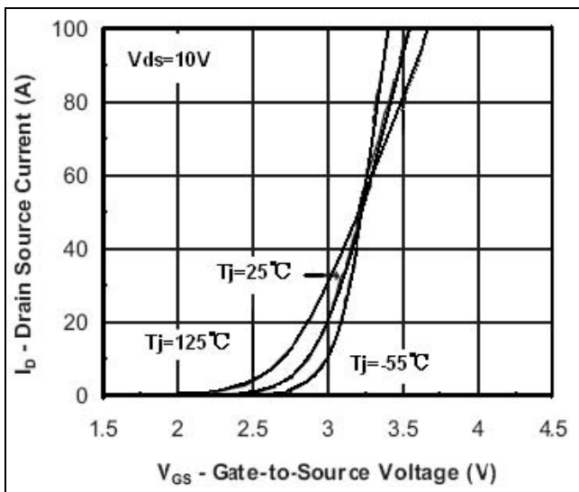
Transfer Characteristic
