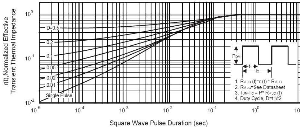
Figure 13: Transient Thermal Impedance Curve
