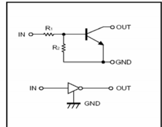
●Equivalent circuit
