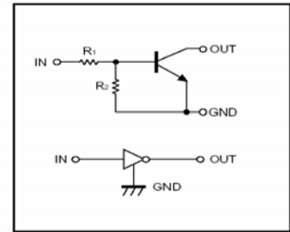
●Equivalent circuit
