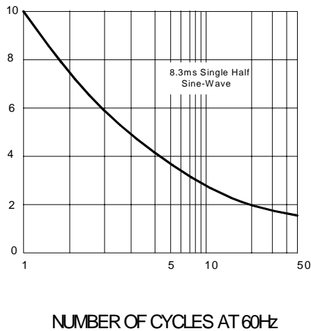
FIG.4 – PEAK FORWARD SURGE CURRENT
