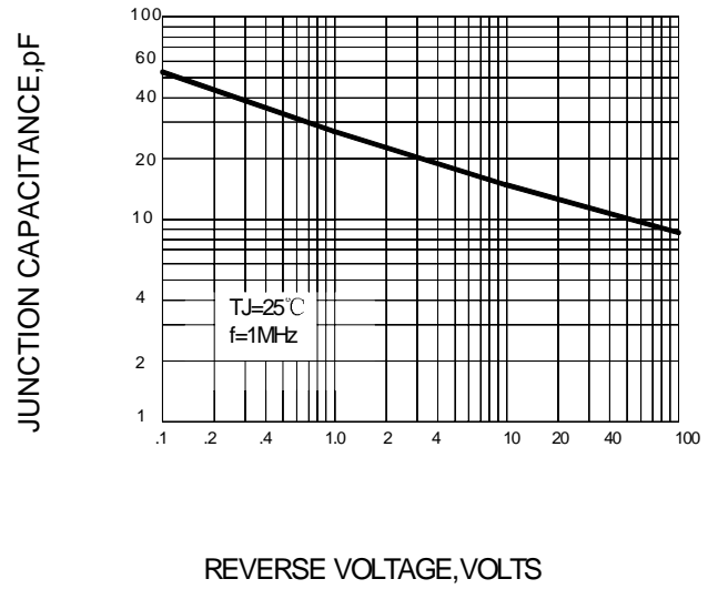
FIG.2 – JUNCTION CHARACTERISTICS
