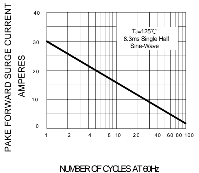
FIG.5 – PEAK FORWARD SURGE CURRENT
