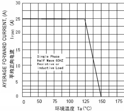
FIG. 1 – MAXIMUM AVERAGE FORWARD CURRENT DERATING
