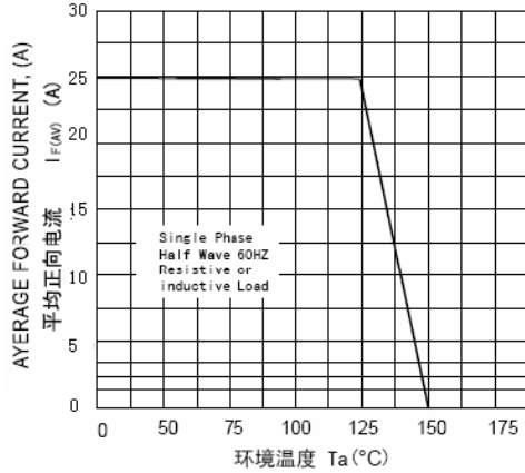
FIG. 1 –MAXIMUM AVERAGE FORWARD CURRENT DERATING
