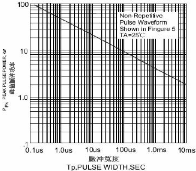
FIG. 5–PULSE RATING CURVE
