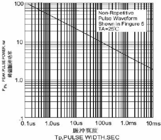
FIG.5–PULSE RATING CURVE
