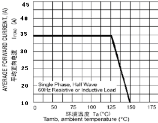
FIG. 1 – 输出电流曲线 FIG. 1 – DERATING CURVE FOR OUTPUT RECTIFIER CURRENT
