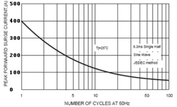
FIG. 2 – 浪涌特性曲线 FIG. 2 – MAXIMUM NON – REPETITIVE PEAK FORWARD SURGE CURRENT
