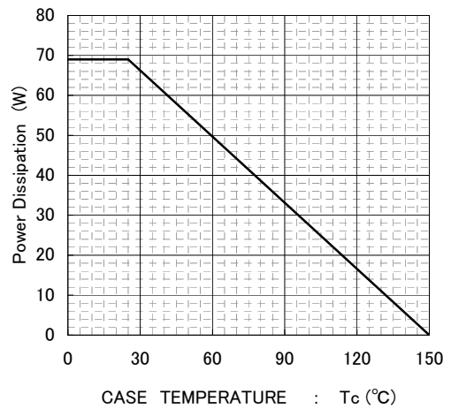
Fig.6 Power Dissipation
