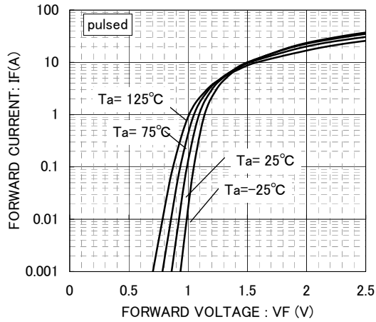
Fig.1 VF-IF CHARACTERISTICS
