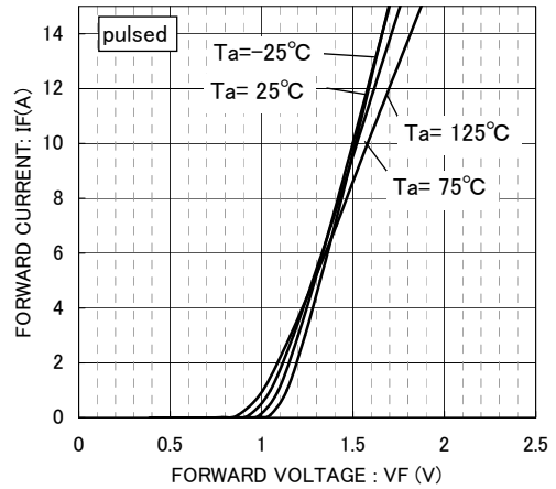
Fig.2 VF-IF CHARACTERISTICS
