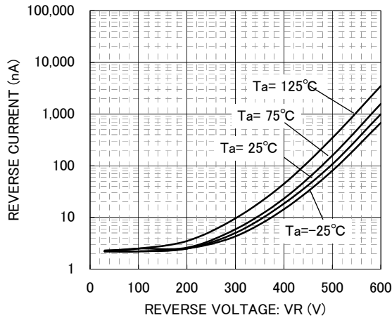
Fig.3 VR-IR CHARACTERISTICS
