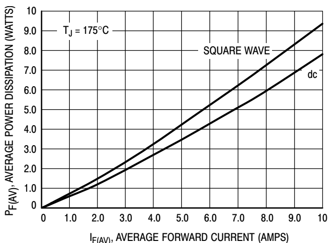
Figure 5. Power Dissipation, Per Leg
