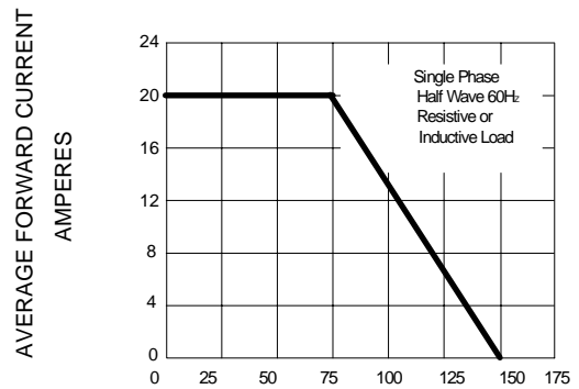
FIG.3 -- FORWARD DERATING CURVE
