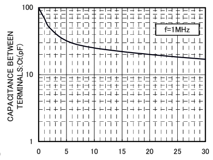
REVERSE VOLTAGE : V_r (V) V_r - C_t CHARACTERISTICS
