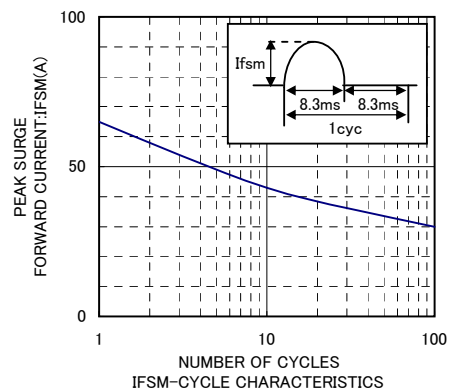
IFSM-CYCLE CHARACTERISTICS
