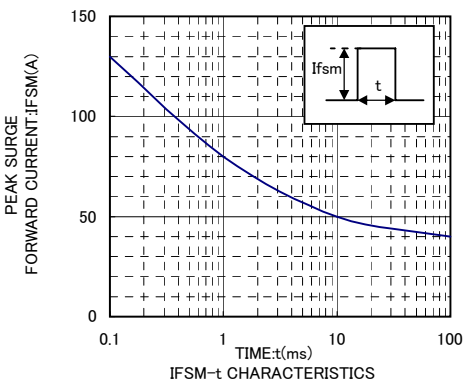
IFSM-t CHARACTERISTICS
