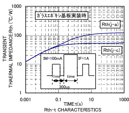
Rth-t CHARACTERISTICS
