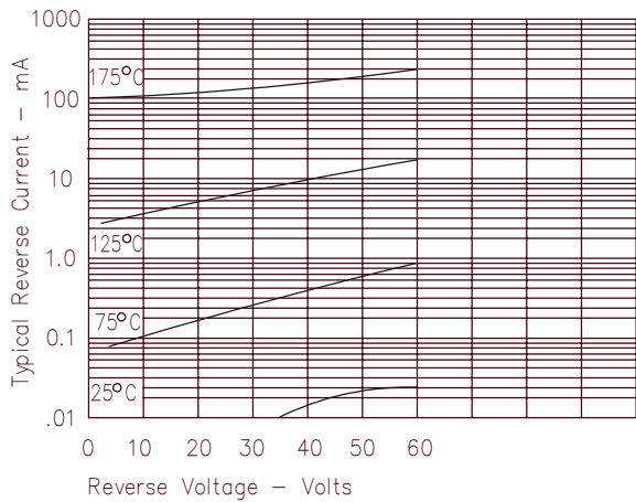
Figure 2 Typical Reverse Characteristics – Per Leg
