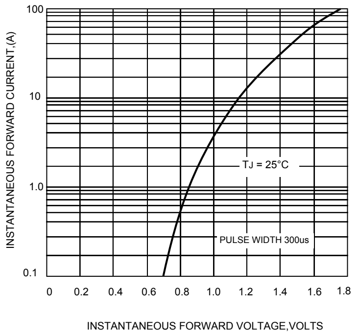
FIG.4-TYPICAL FORWARD CHARACTERISTICS
