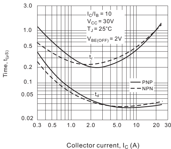
Fig.3 Turn-on time
