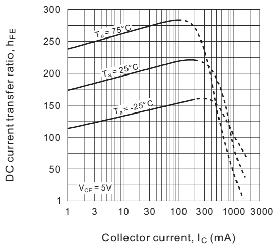
Fig.5 DC current transfer ratio vs. collector current
