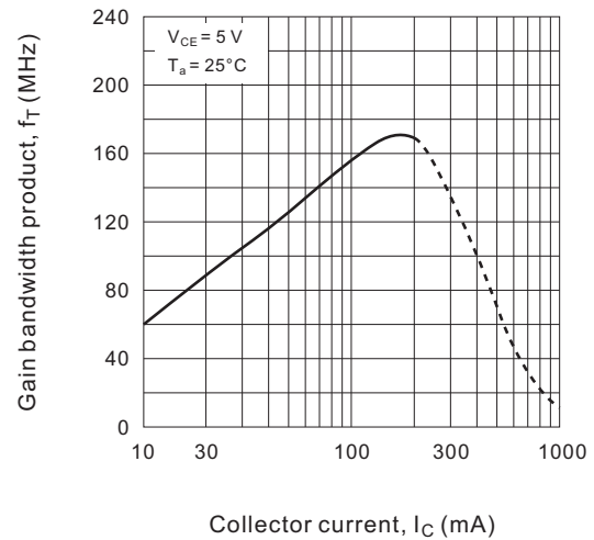
Fig.8 Gain bandwidth product vs. collector current
