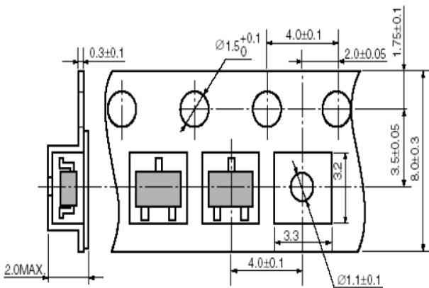
Tape Dimension
