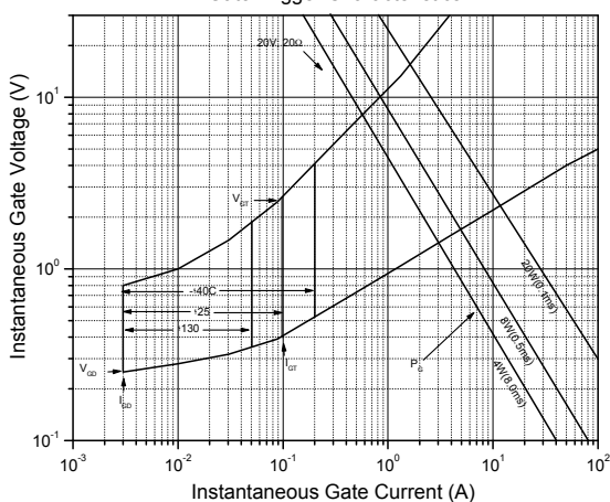
Gate Trigger Characteristics
