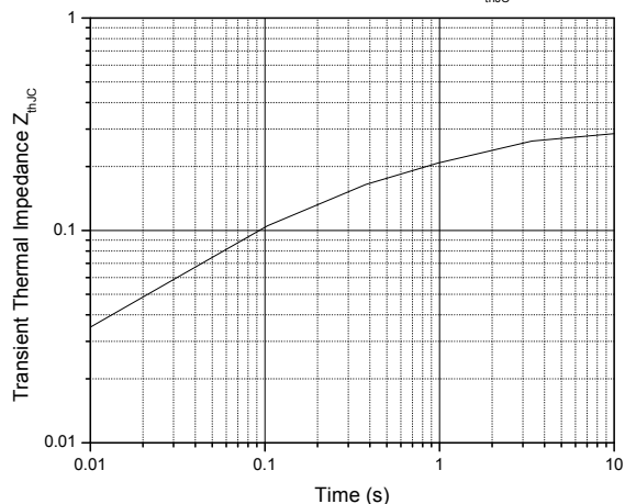
Transient Thermal Impedance Z_{thJC}
