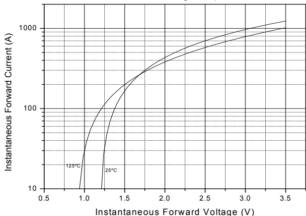
Forward Voltage Drop
