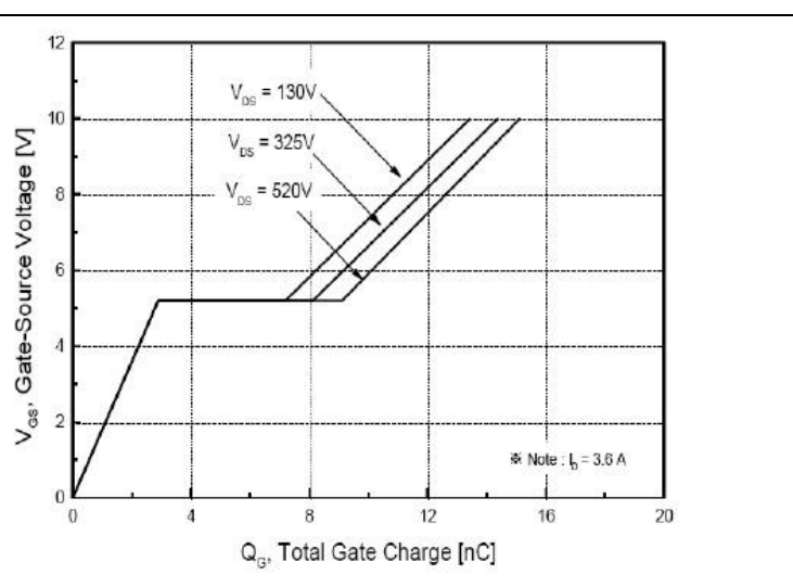
FIG.6-GATE CHARGE CHARACTERISTICS
