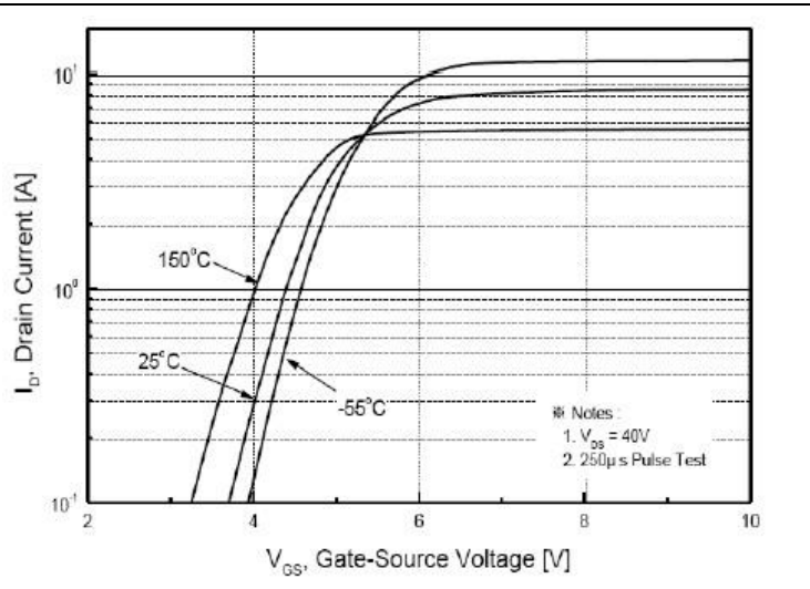
FIG.2-TRANSFER CHARACTERISTICS
