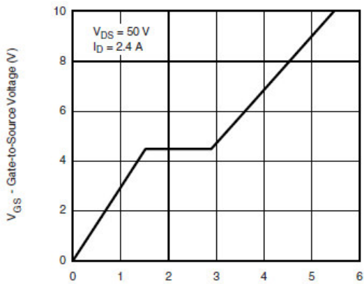
Gate Charge
