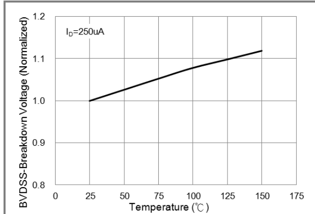
Fig.8 BV_{DSS} vs. Junction Temperature
