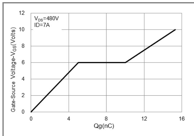
Fig.6 Gate Charge
