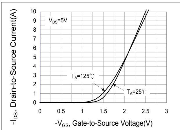
Fig.3 Transfer Characteristic
