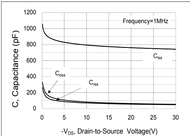
Fig.1 Capacitance Characteristic
