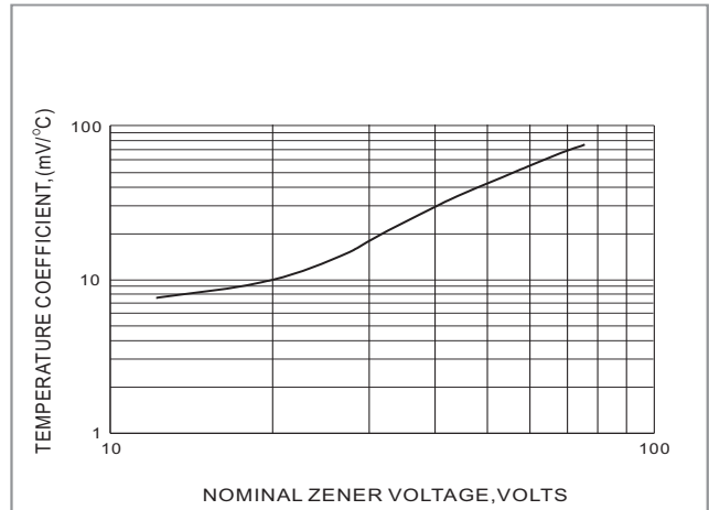
Fig.2 TEMPERATURE COEFFICIENTS
