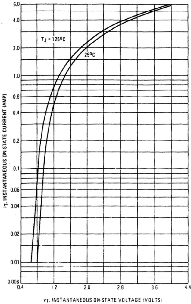
FIGURE 9 – MAXIMUM ON STATE CHARACTERISTICS
