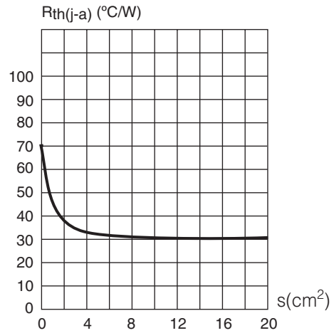
Fig. 10: D2PAK thermal resistance junction to ambient versus copper surface under tab (printed circuit board copper thickness: 35µ)
