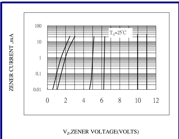
Fig.3A-V Z =2.0 THRU 11.0 VOLTS
