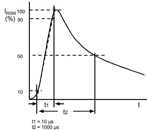
Fig.4 - Non-Repetitive peak reverse current pulse definition
