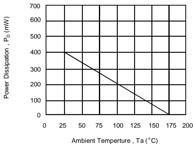
Derating Curve
