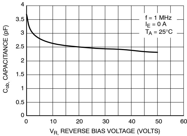
Figure 54. Output Capacitance
