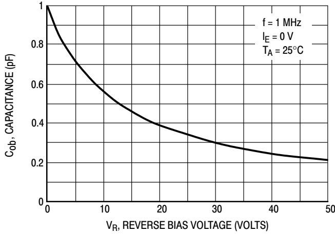
Figure 14. Output Capacitance
