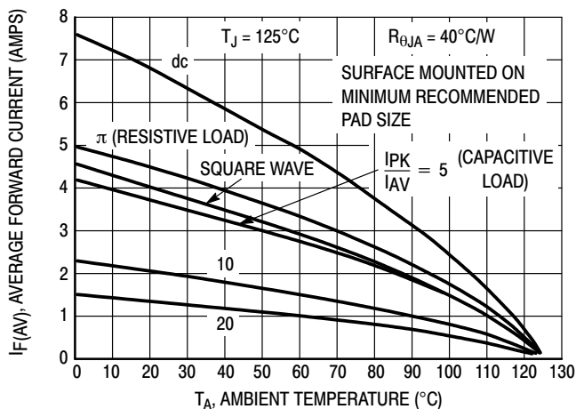
Figure 7. Current Derating
