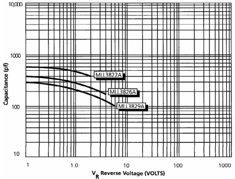
FIGURE 2 Typical Capacitance vs. Reverse Voltage
