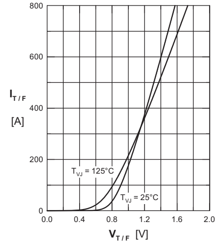
Fig. 1 Forward characteristics
