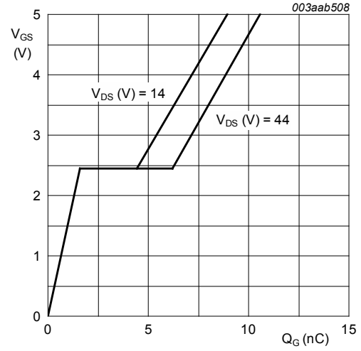
Fig. 8. Gate-source voltage as a function of gate charge; typical values
