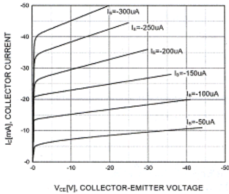
Static Characteristic
