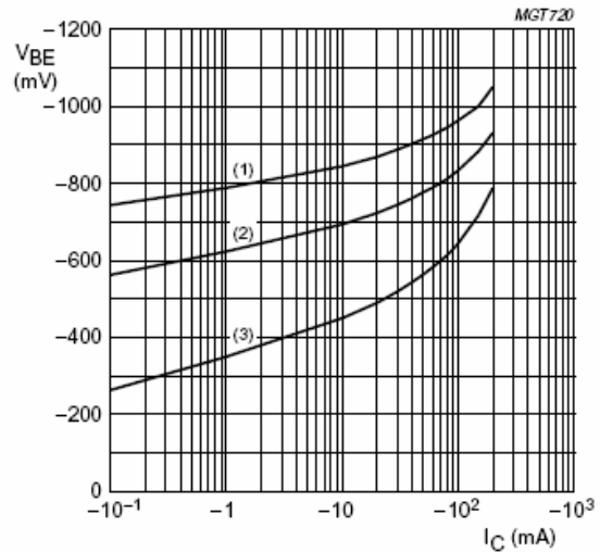
BC857CW; V_{CE} = -5 V.
