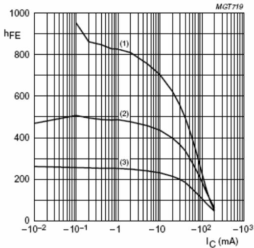
BC857CW; V_{CE} = -5 V.
