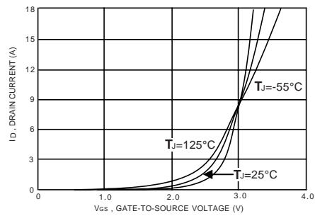
Figure 2. Transfer Characteristics
