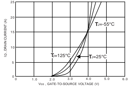
Figure 2. Transfer Characteristics
