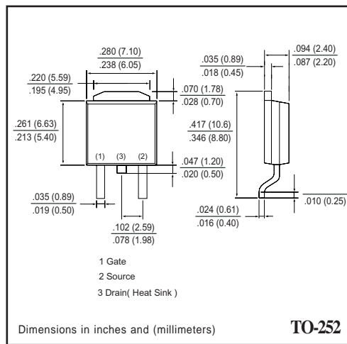
D-PAK(TO-252)
